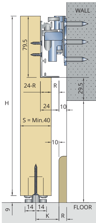
Wall fitting positioning with skirting
