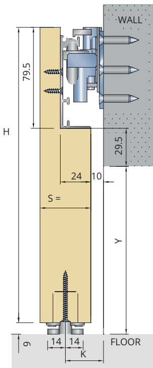
Wall fitting positioning without skirting
